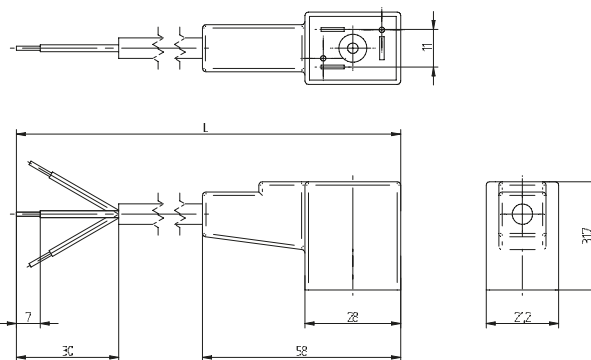
ST 22 L 5000/ST 222 V __ L 1500
